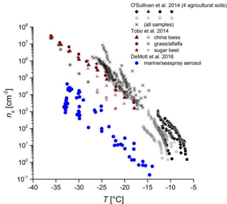
FIG. 1-6. Ice nucleation active site densities n_s as a function of temperature for H_2O_2 (hydrogen peroxide) treated (lighter-shaded symbols) and untreated (dark symbols) agricultural soil dusts in comparison to the n_s of marine aerosol. Differences between various black symbols are for organic content (OC). High OC (12.7 wt%)
