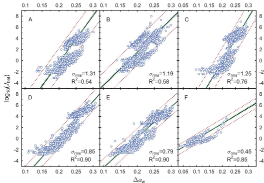
Fig. 3 The decadal log of the heterogeneous ice nucleation rate coefficients, \log_{10}(U_{het}) , are shown as a function of \Delta a_w for individually analysed freezing events, initiated by the different IN types investigated in this study and previous work. 41,43,57,66,73,75,78,95 \log_{10}(U_{het}) are shown for (A) Nannochloris atomus , (B) Thalassiosira pseudonana , (C) Pahokee Peat, (D) Leonardite, (E) Illite, and (F) 1-nonadecanol. The solid black line is a linear fit where dashed green and red lines represent confidence intervals and prediction bands at 95% level. The root mean square error, \sigma_{rms} , and the adjusted coefficient of determination, R^2 , are given in each panel.
