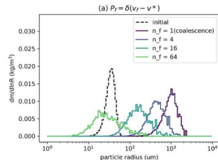
Figure 7. Sensitivity to fragmentation function of PSDs
